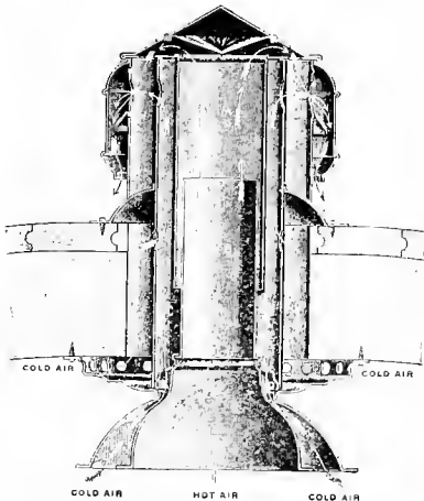
Fig. 3277. IMPROVED COMBINATION SMOKE-BELL AND VENTILATOR.
